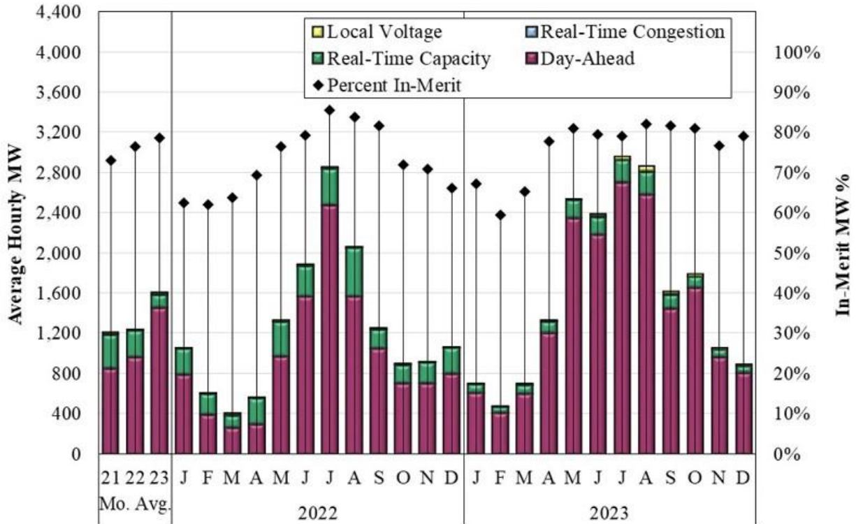
Figure A65: Dispatch of Peaking Resources By Commitment Reason, 2022–2023
