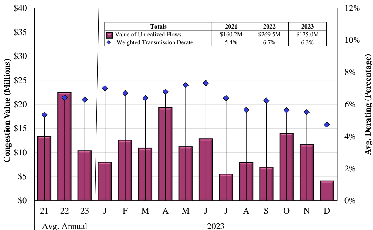
Figure A85: Value of Unrealized Transmission Flows from Limit Control Derates
