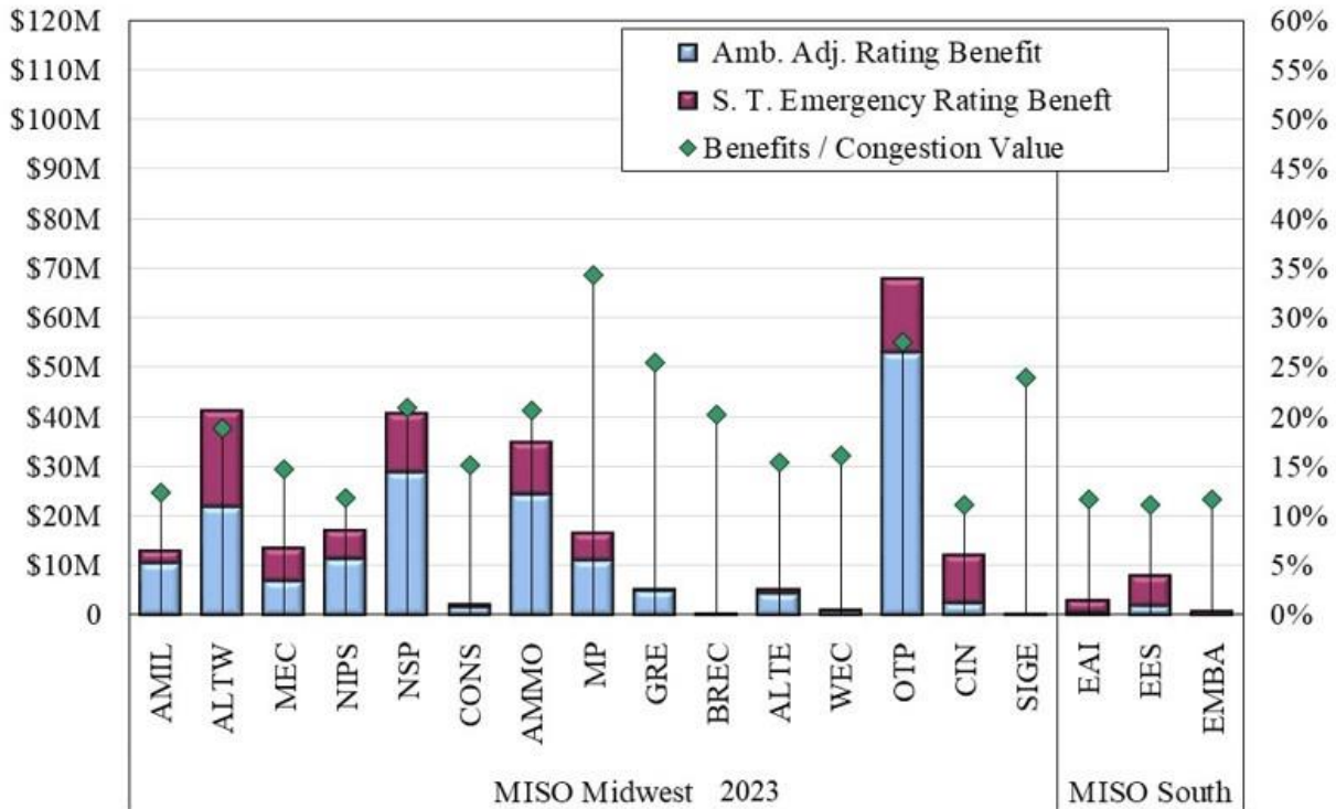
Figure A84: Area-Specific Savings Potential of Ratings Enhancement
