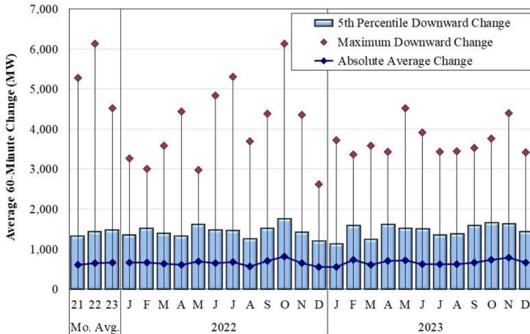
Figure A69: Wind Generation Volatility 2022–2023
