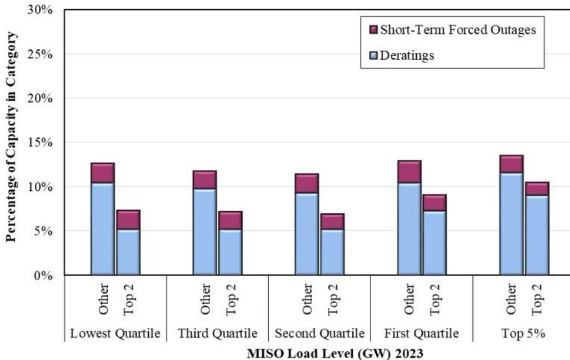
Figure A151: Real-Time Deratings and Forced Outages Central Region, 2023
