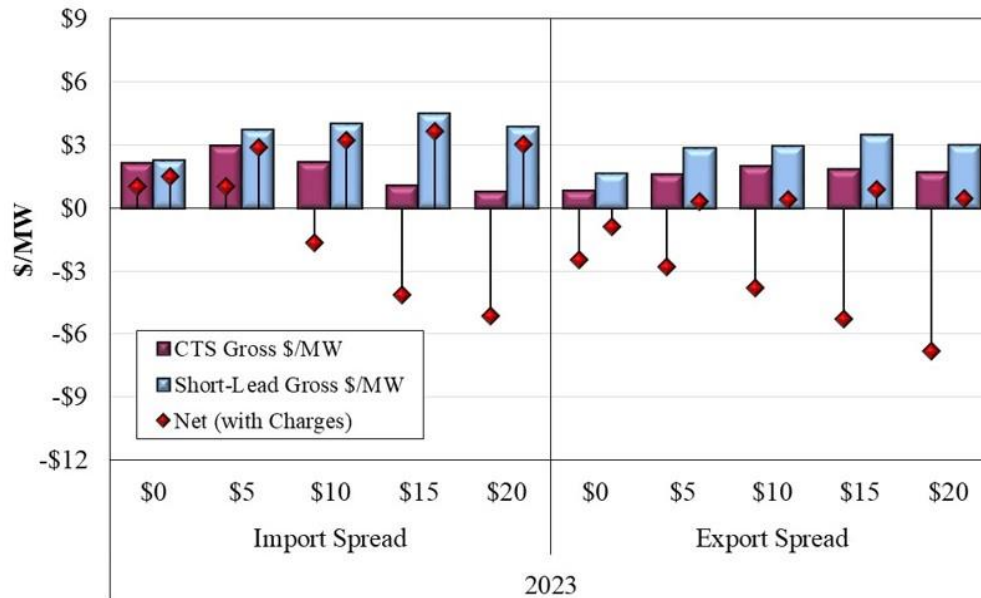
Figure A129: CTS Versus Traditional NSI Scheduling 2023
