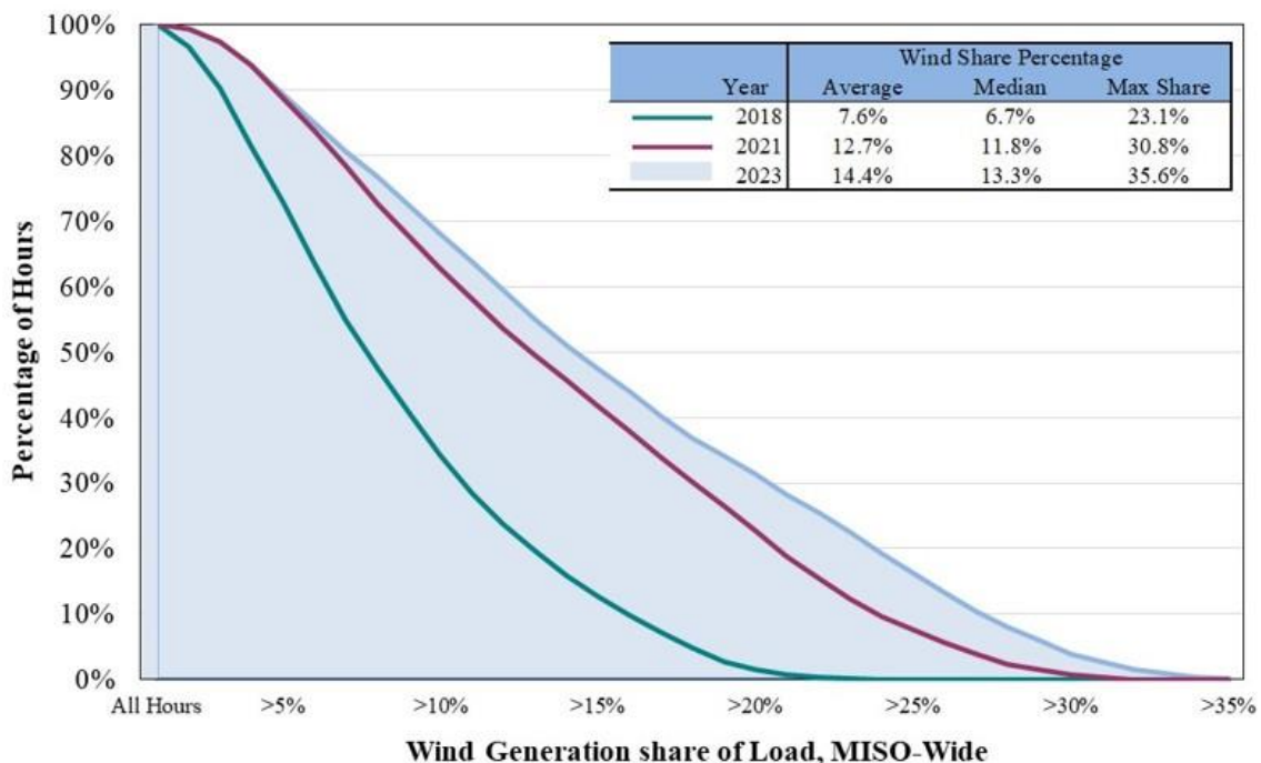
Figure A13: Share of MISO Load Served by Wind Generation Over Time 2018–2023
