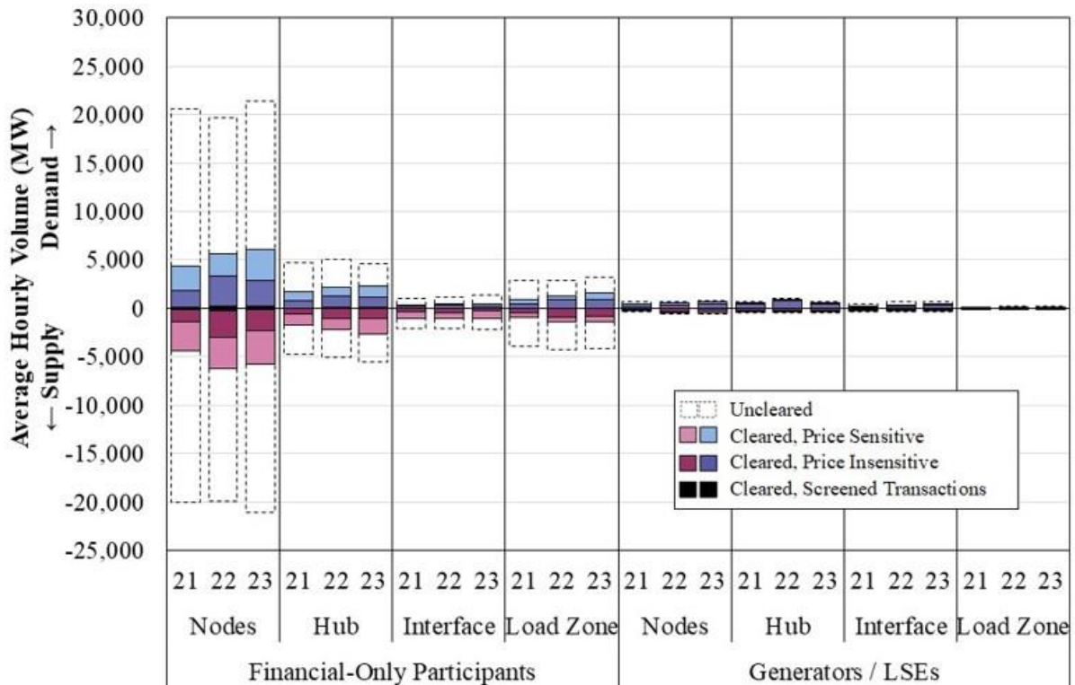
Figure A39: Virtual Transaction Volumes by Participant Type and Location 2021–2023
