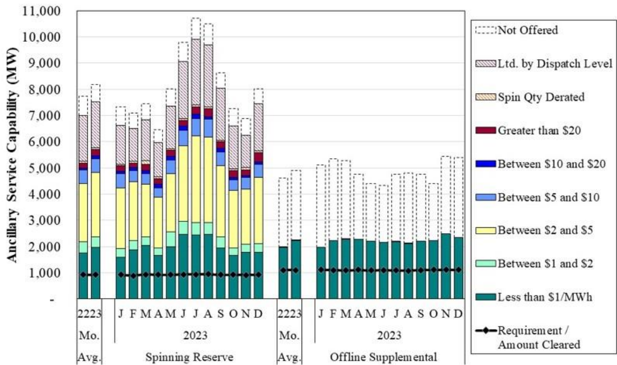
Figure A11: Contingency Reserve Offers and Scheduling 2023
