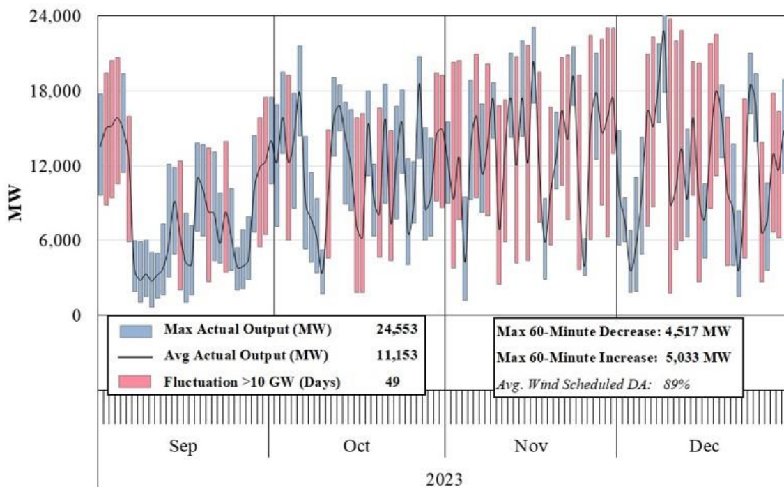
Figure A16: Daily Range of Wind Generation Output September – December 2023
