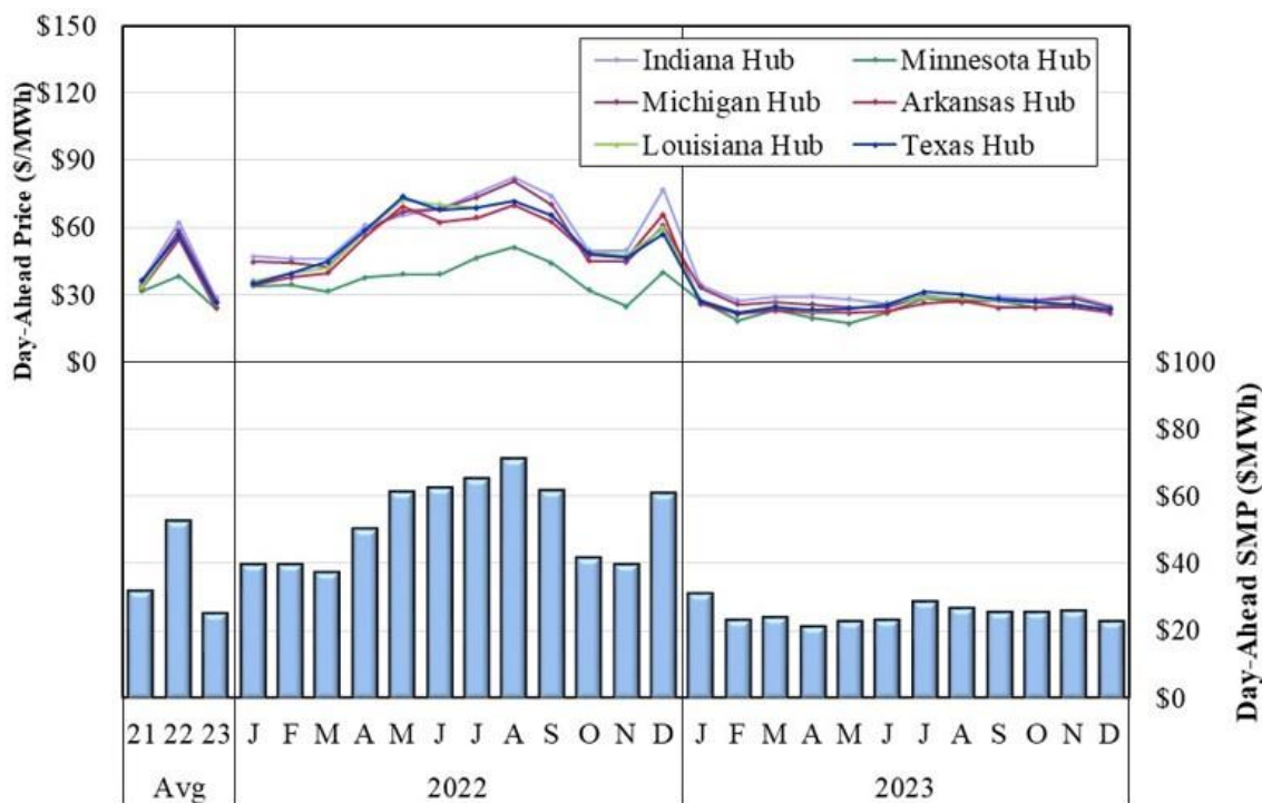
Figure A21: Day-Ahead Hub Prices and SMP Off-Peak Hours, 2022–2023
