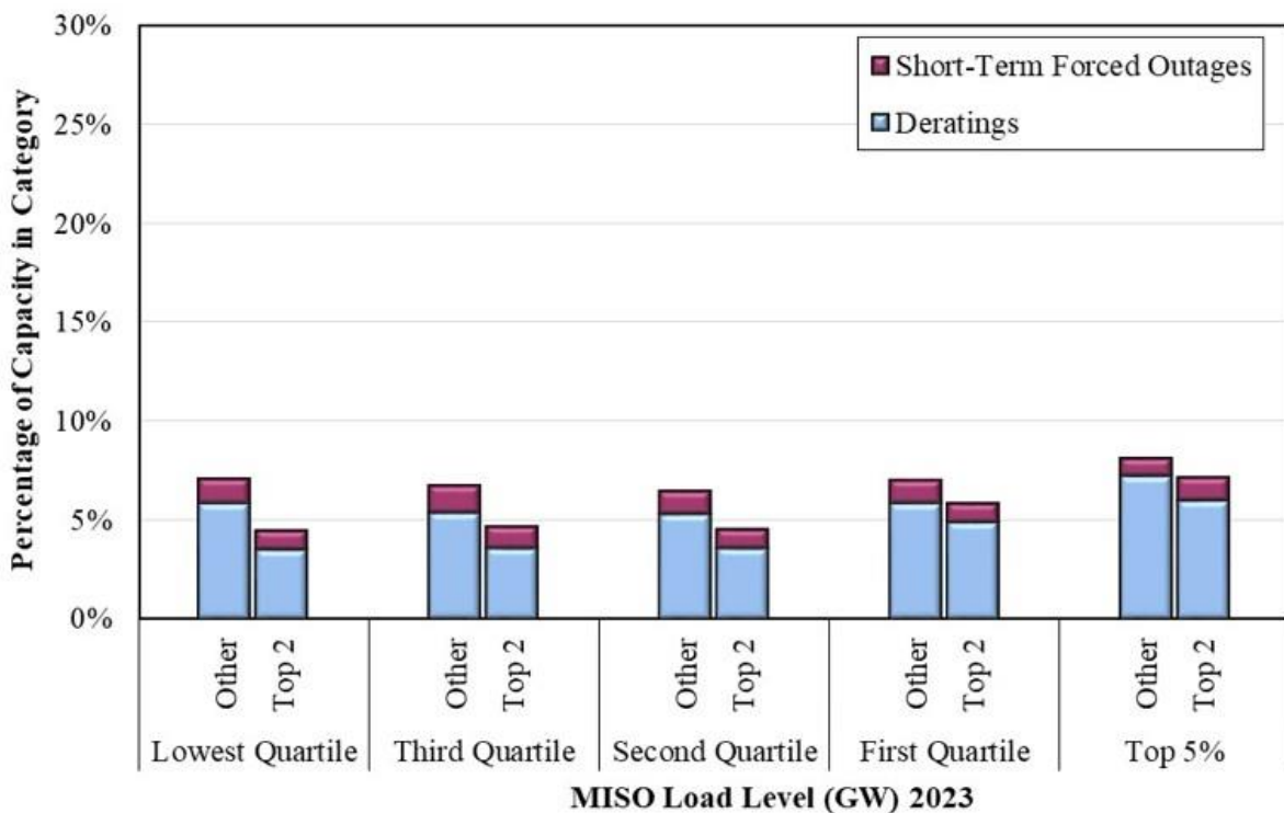
Figure A153: Real-Time Deratings and Forced Outages North Region, 2023
