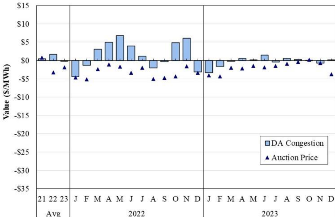
Figure A113: Comparison of FTR Auction Prices and Congestion Value Louisiana Hub, 2022–2023: Off-Peak Hours
