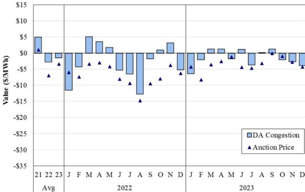
Figure A116: Comparison of FTR Auction Prices and Congestion Value Texas Hub, 2022–2023: Peak Hours
