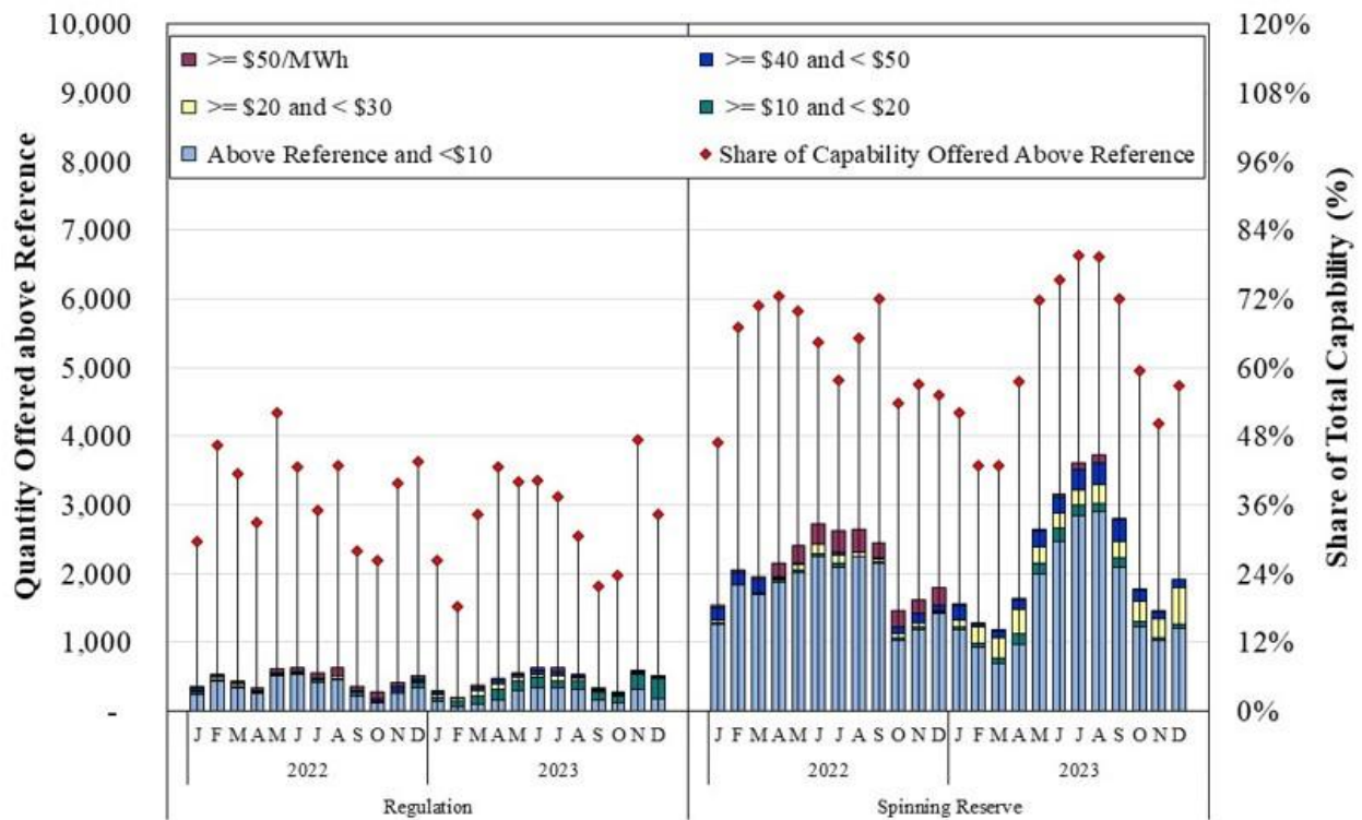
Figure A150: Ancillary Services Market Offers MISO South, 2022–2023
