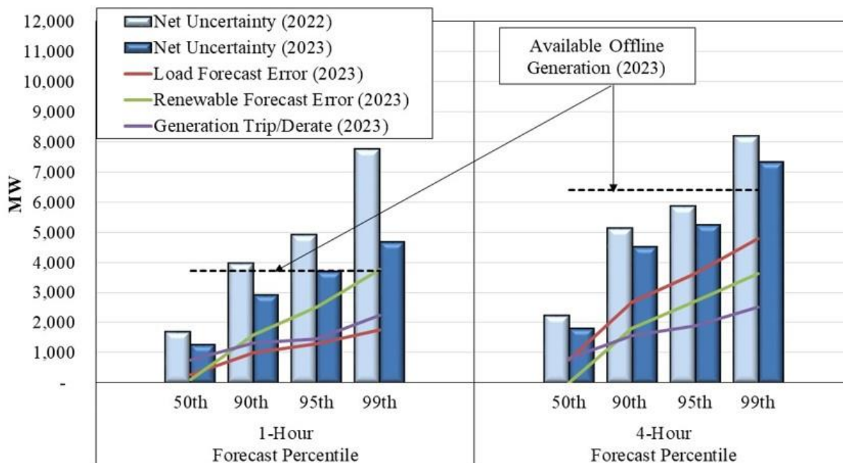
Figure A18: Uncertainty and MISO’s Operating Requirements January 2022 to December 2023
