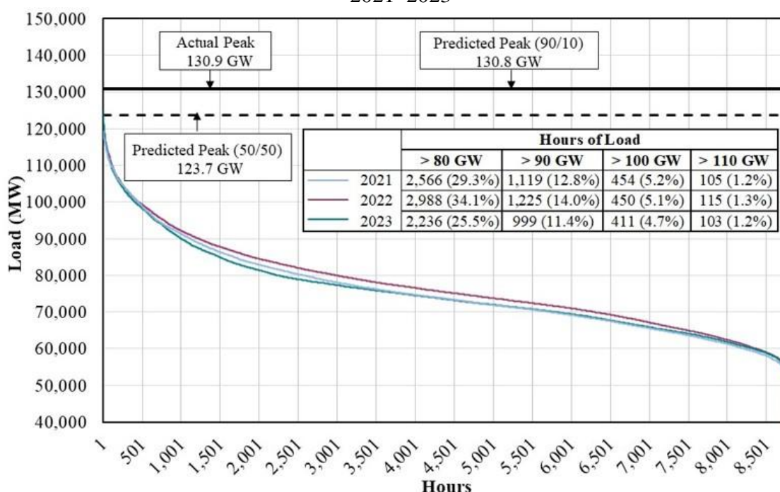
Figure A7: Load Duration Curves and 2023 Peak Load 2021–2023
