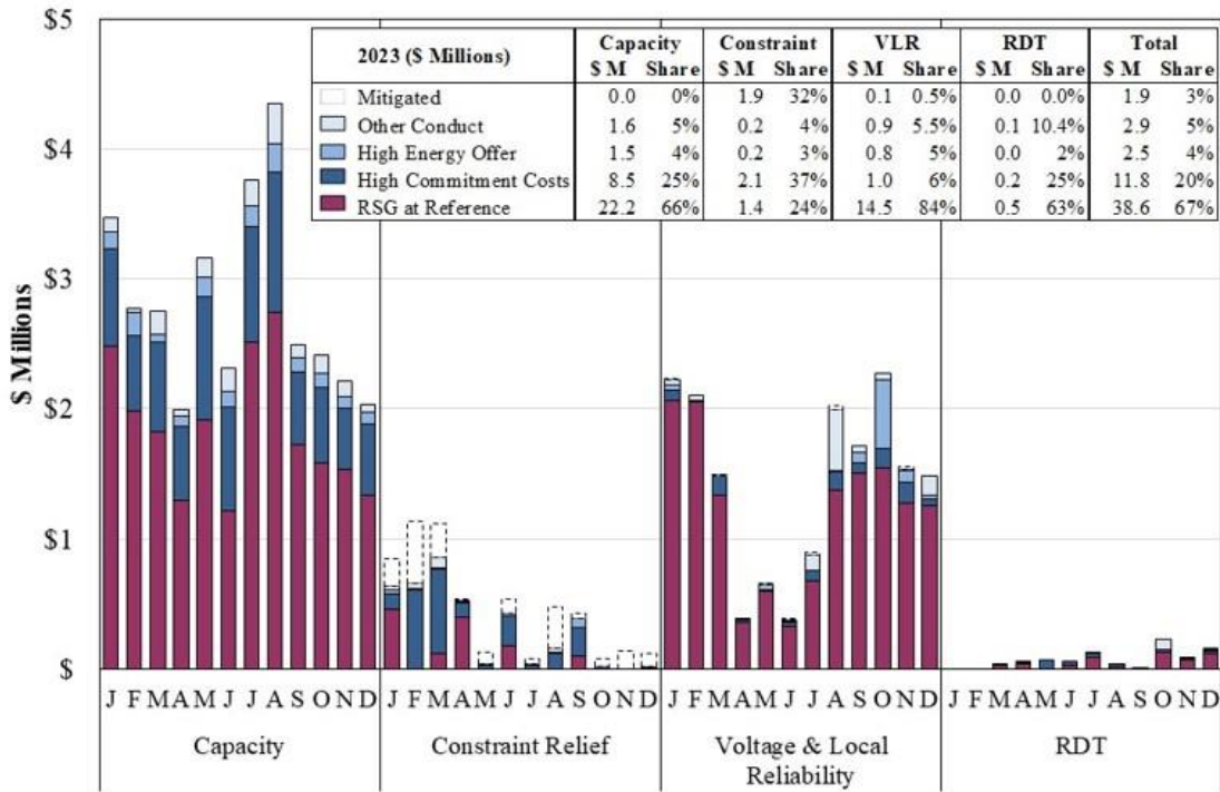
Figure A146: Real-Time RSG Payments by Conduct Midwest Region, by Commitment Reason, 2023
