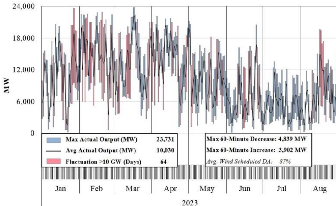
Figure A15: Daily Range of Wind Generation Output January – August 2023
