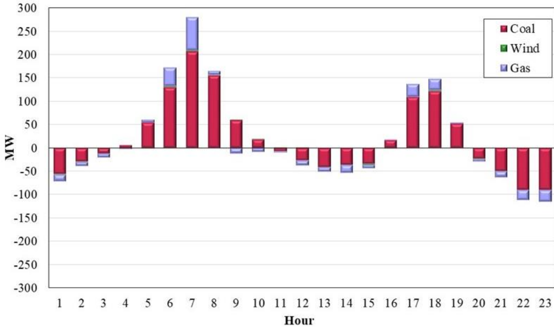
Figure A62: 60-Minute Deviation by Fuel and Hour Winter 2023
