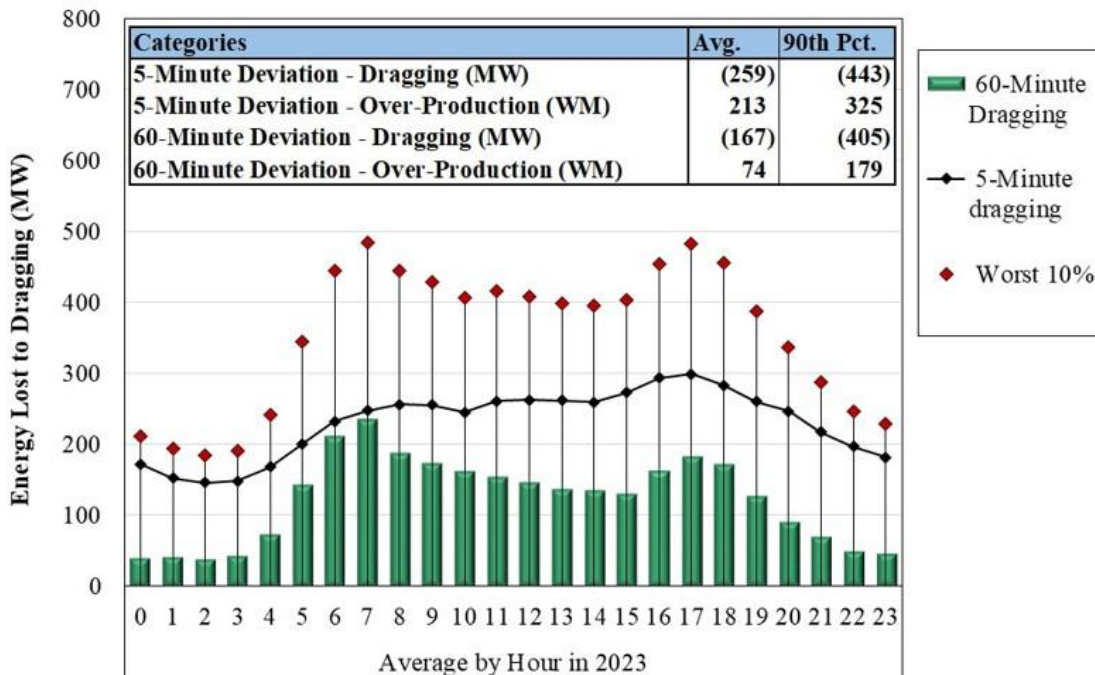
Figure A63: Hourly 60-Minute Deviations by Type of Conduct 2023
