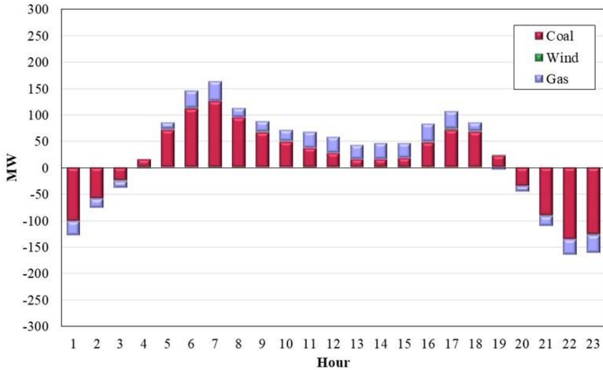
Figure A61: 60-Minute Deviation by Fuel and Hour Summer 2023
