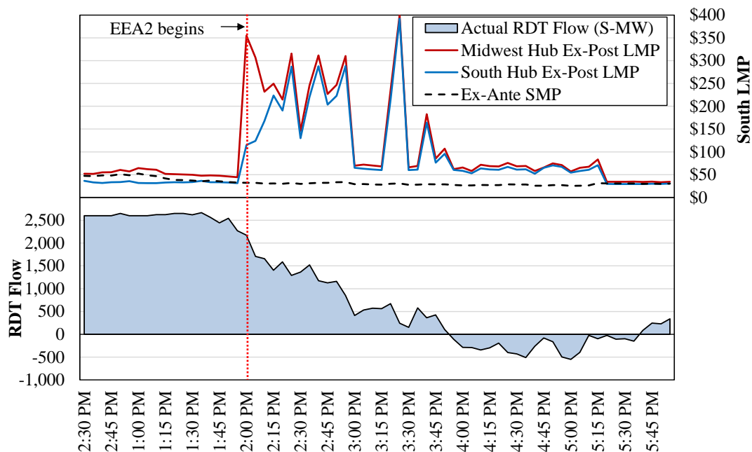
Figure A47: Actual EEA2 Pricing and RDT Flows June 10, 2021
