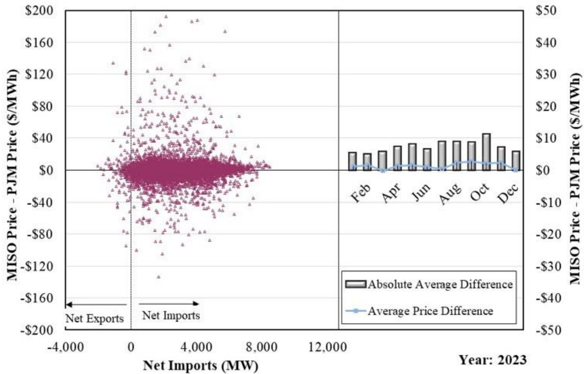
Figure A132: Real-Time Prices and Interface Schedules PJM and MISO, 2023
