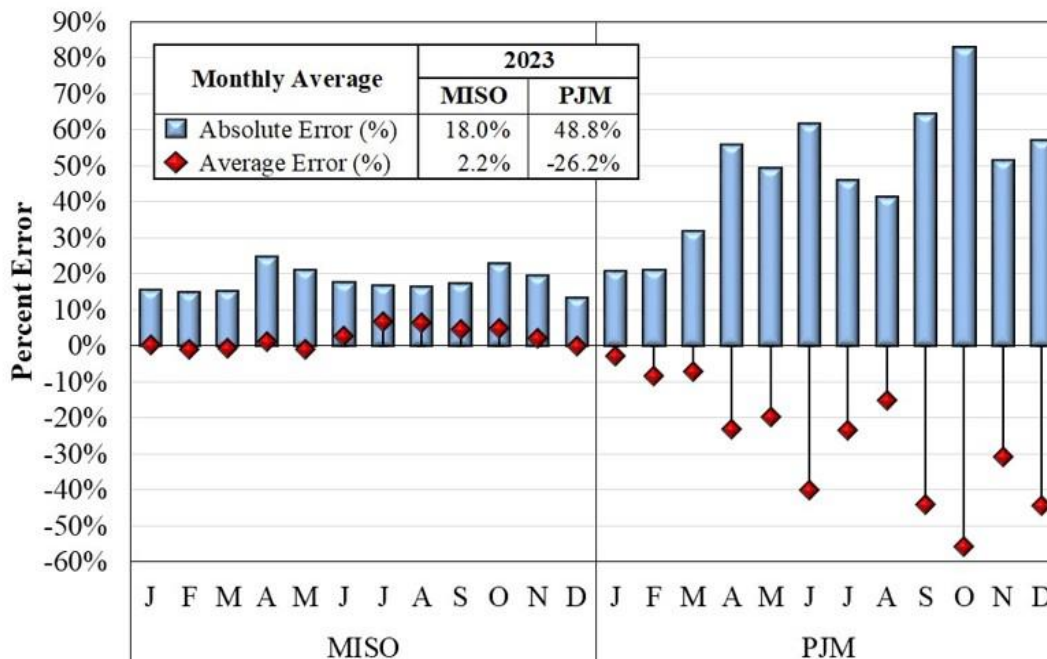
Figure A130: MISO and PJM CTS Forecast Errors 2023
