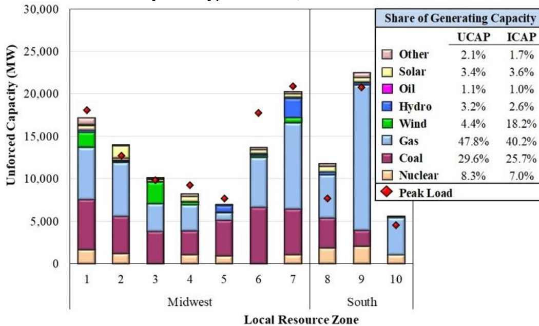
Figure A118: Distribution of Existing Generating Capacity By Fuel Type and Zone, December 2023
