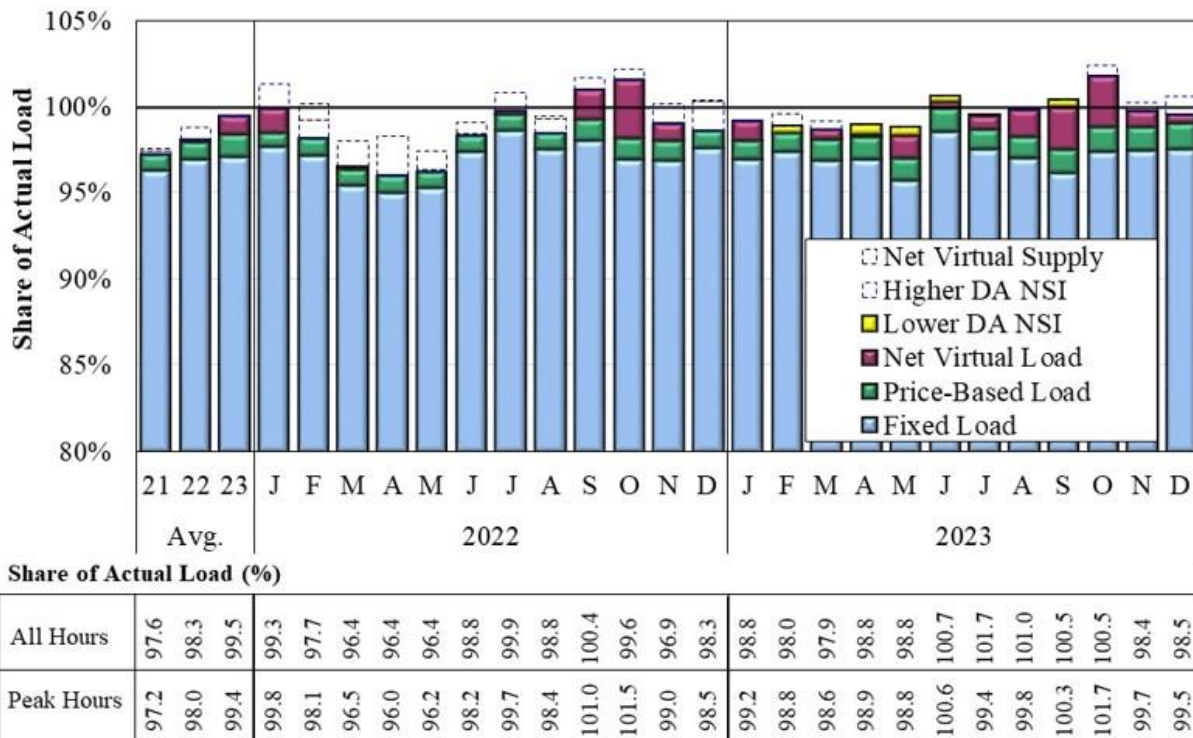
Figure A30: MISO Midwest Day-Ahead Scheduled Versus Actual Loads 2022–2023, Daily Peak Hour
