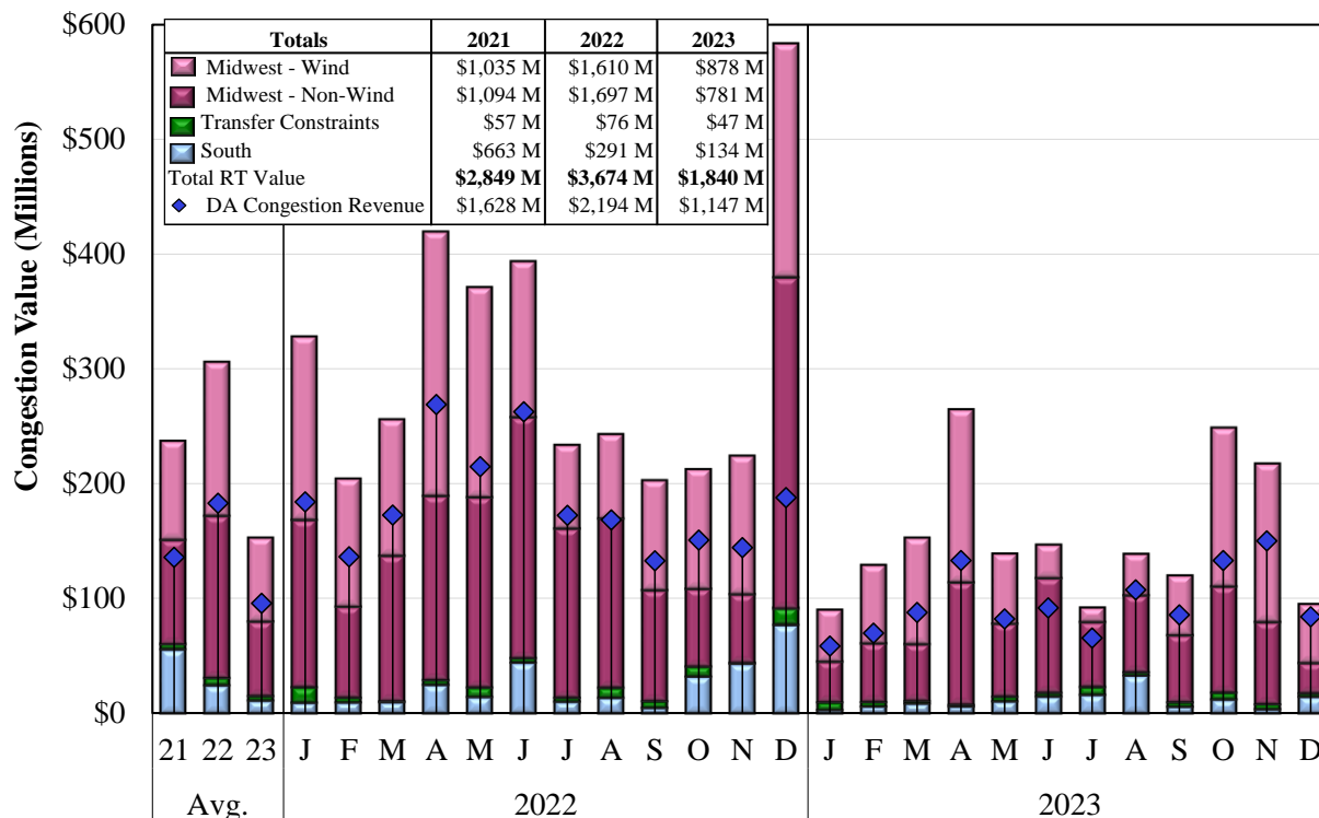
Figure A72: Value of Real-Time Congestion by Coordination Region 2022–2023
