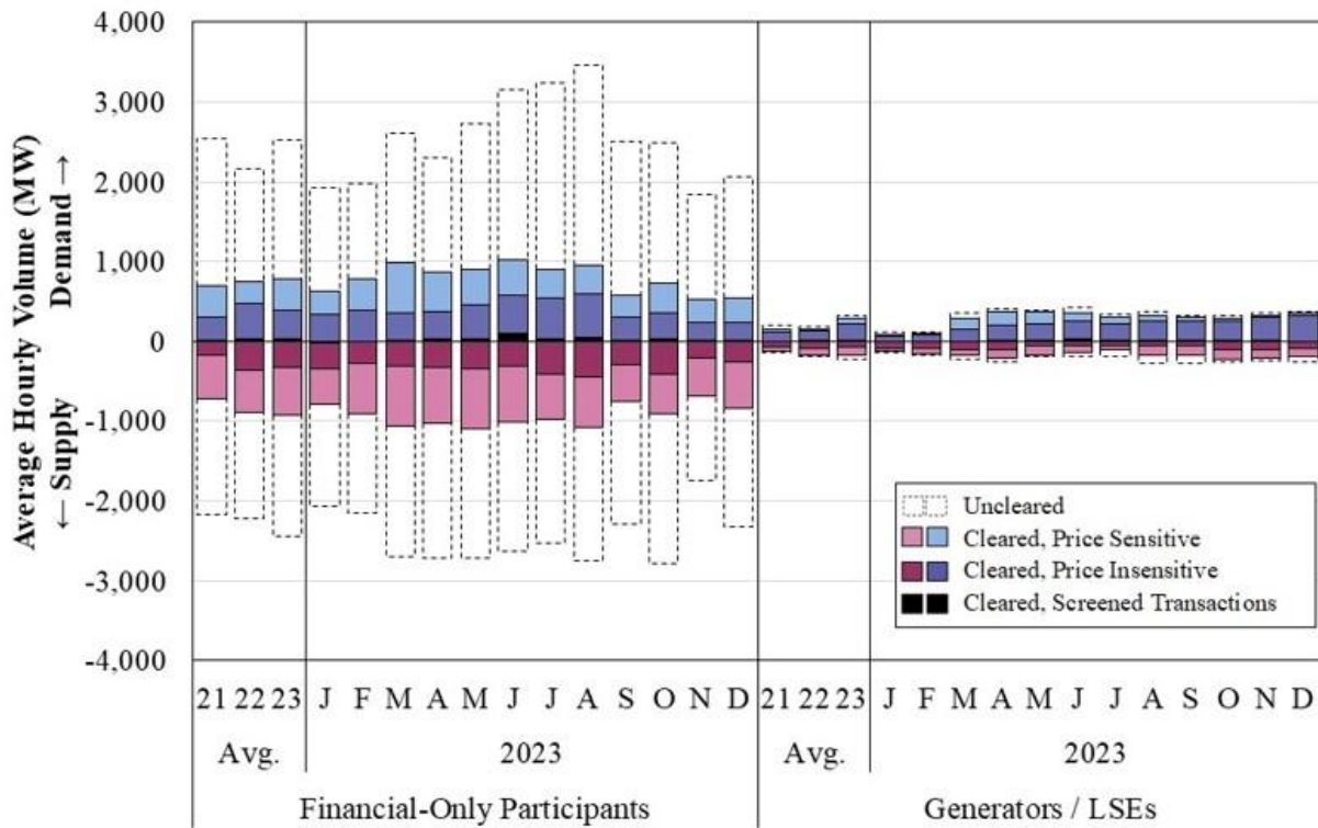
Figure A38: Virtual Transaction Volumes by Participant Type MISO South, 2023
