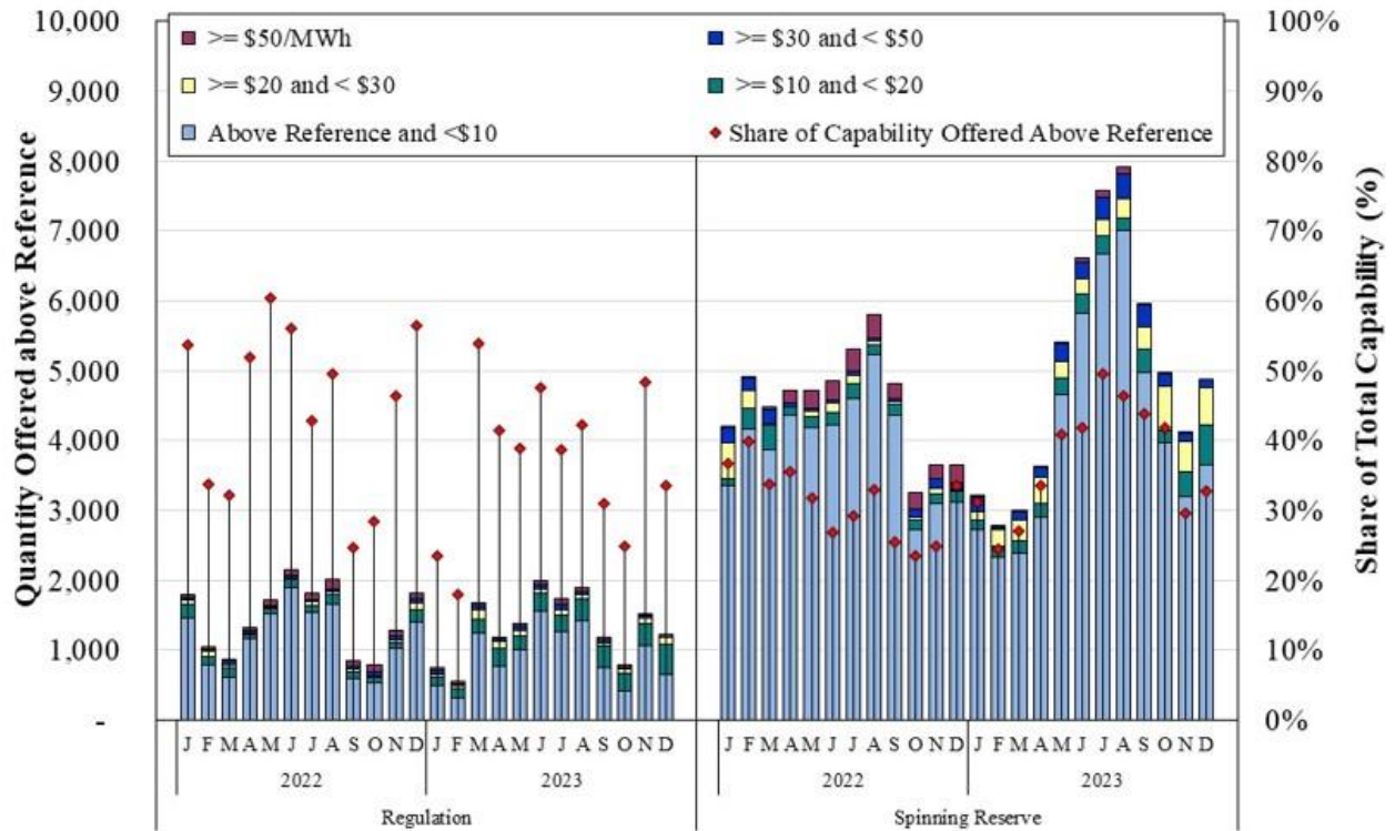
Figure A148: Ancillary Services Market Offers 2022–2023
