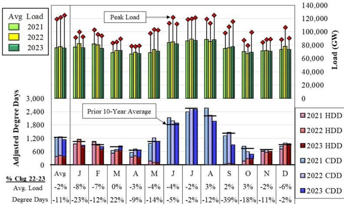
Figure A8: Heating and Cooling Degree-Days 2021–2023
