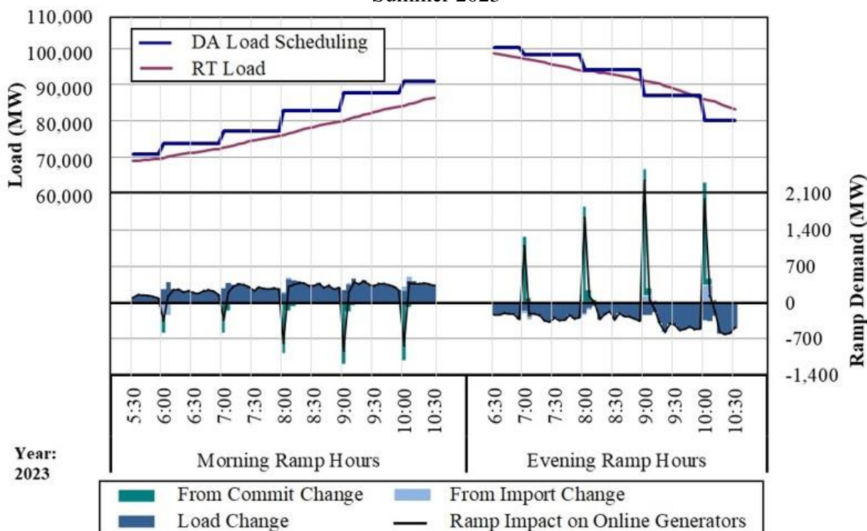
Figure A33: Ramp Demand Impact of Hourly Day-Ahead Market Summer 2023
