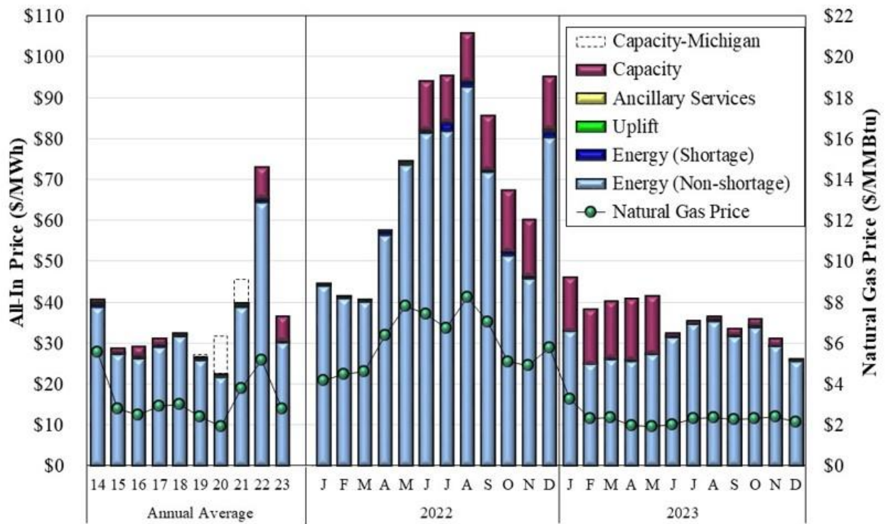
Figure A1: All-In Price of Electricity 2022–2023
