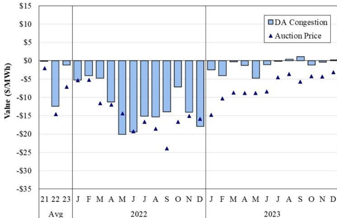
Figure A109: Comparison of FTR Auction Prices and Congestion Value Minnesota Hub, 2022–2023: Off-Peak Hours
