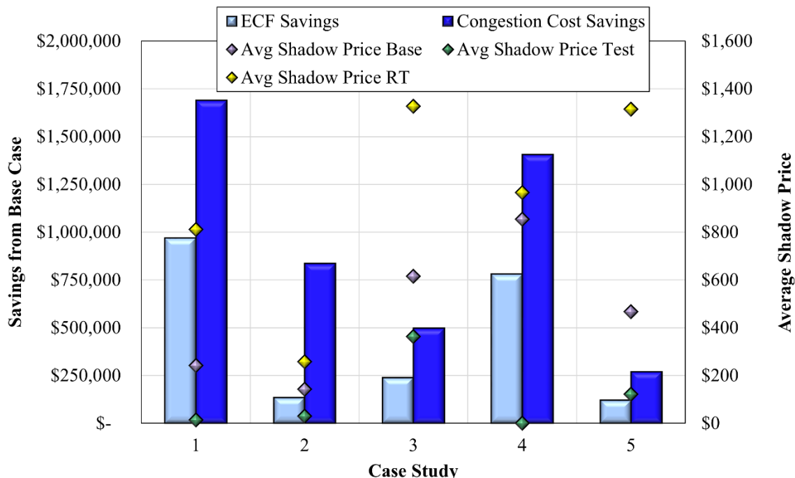
Figure A79: Congestion Savings and Shadow Price Changes
