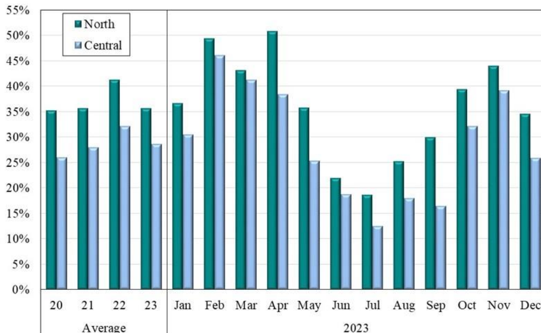
Figure A70: Wind Generation Capacity Factors
