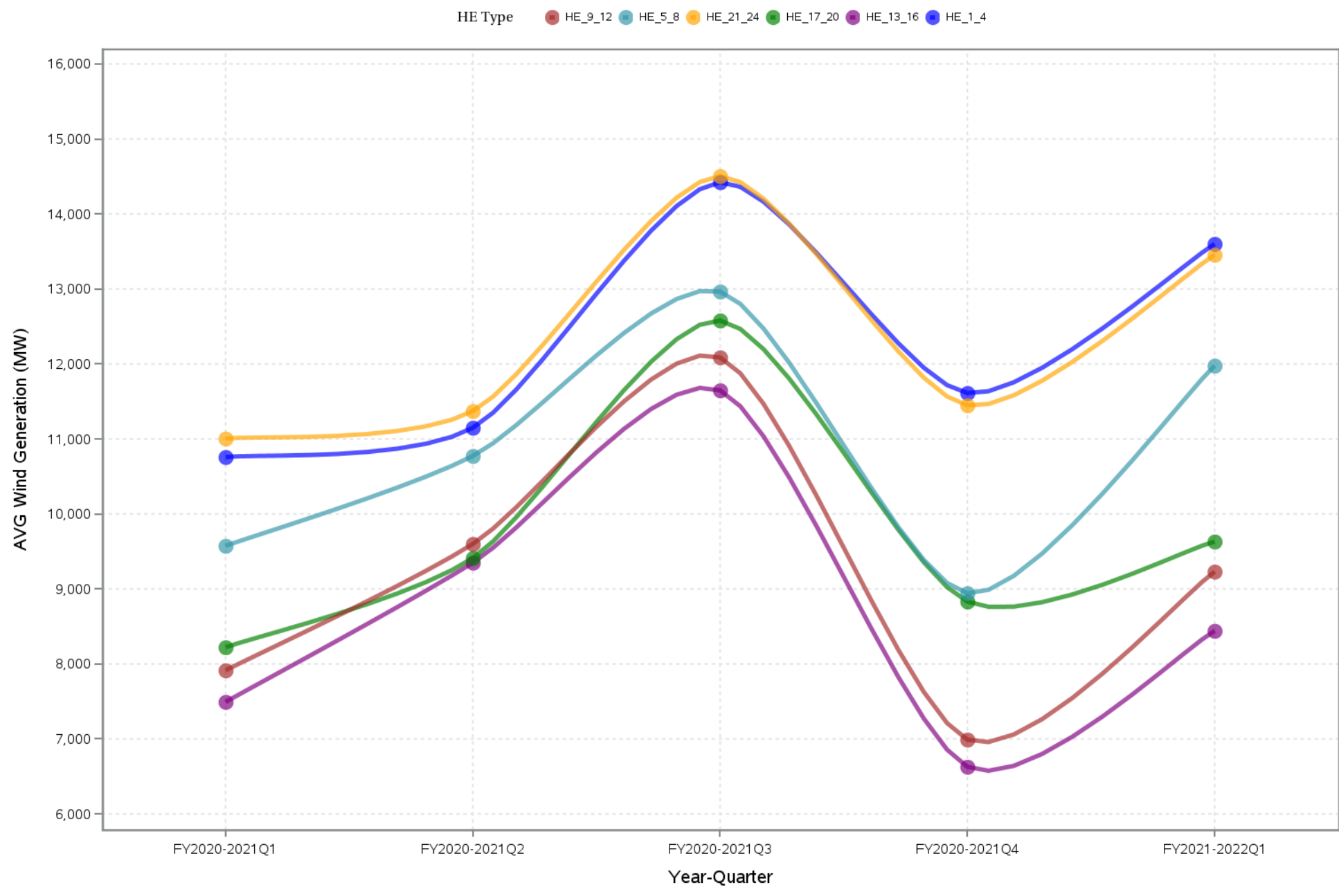
Quarterly Average of Wind Generation by Hour Ending
