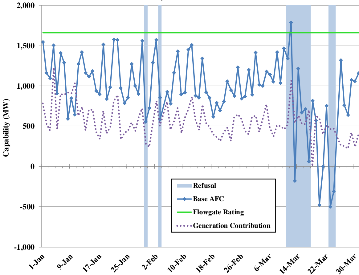
Figure 9: Base AFC – Katoma Reactor to Oconee 500 kV (DUK) January 2017 - March 2017
