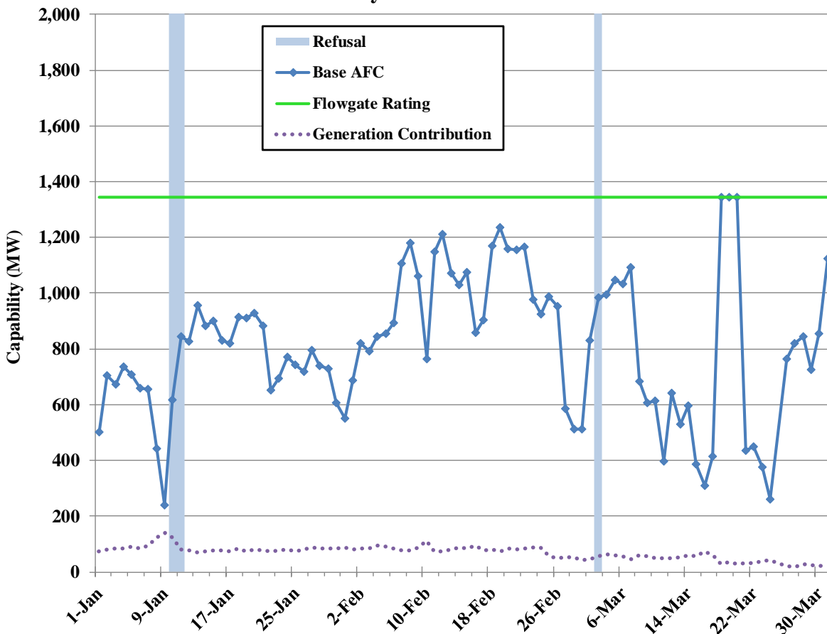
Figure 11: Base AFC –McIntosh 500/230 kV (SOCO) January 2017 - March 2017
