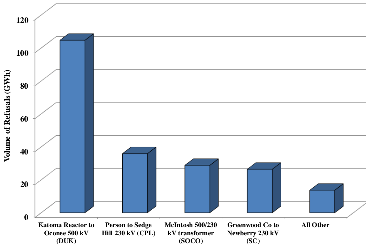
Figure 8: Key Flowgates Linked to Current TSR Refusals January 2017 – March 2017
