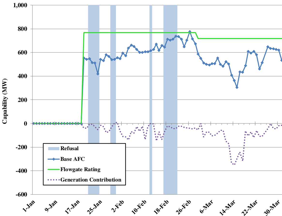
Figure 10: Base AFC – Person to Sedge Hill 230 kV (CPL) January 2017 - March 2017
