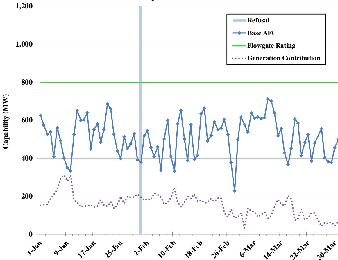
Figure 12: Base AFC – Greenwood Co to Newberry 230kV (SC) January 2017 - March 2017
